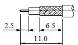
STRIPPING DIMENSION
